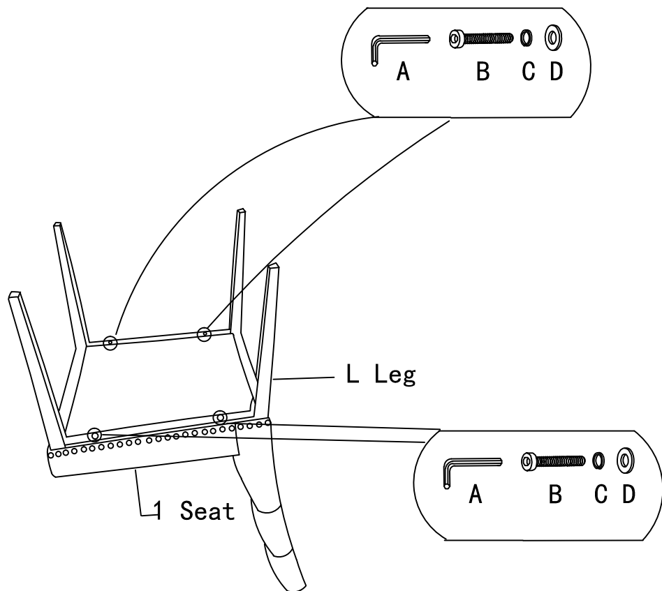
Complete Assembly
